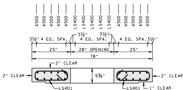
SECTION C-C
