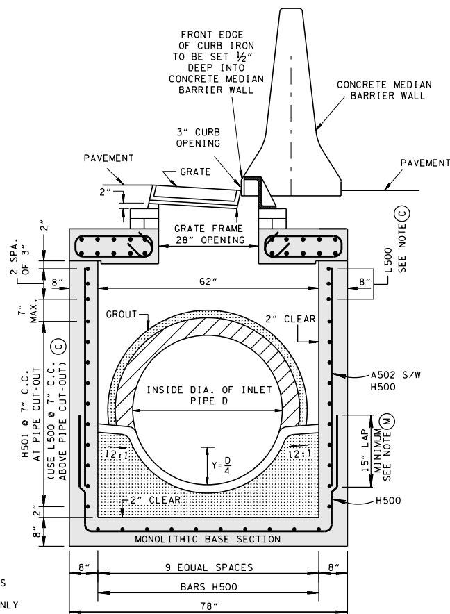
SECTION B-B
